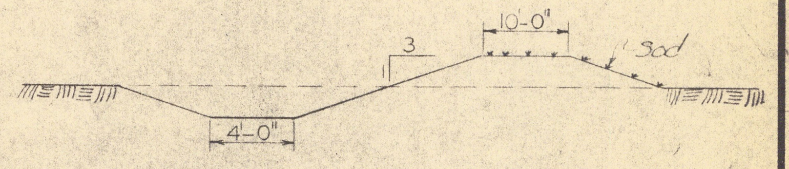
DIKE TYPICAL SECTION
