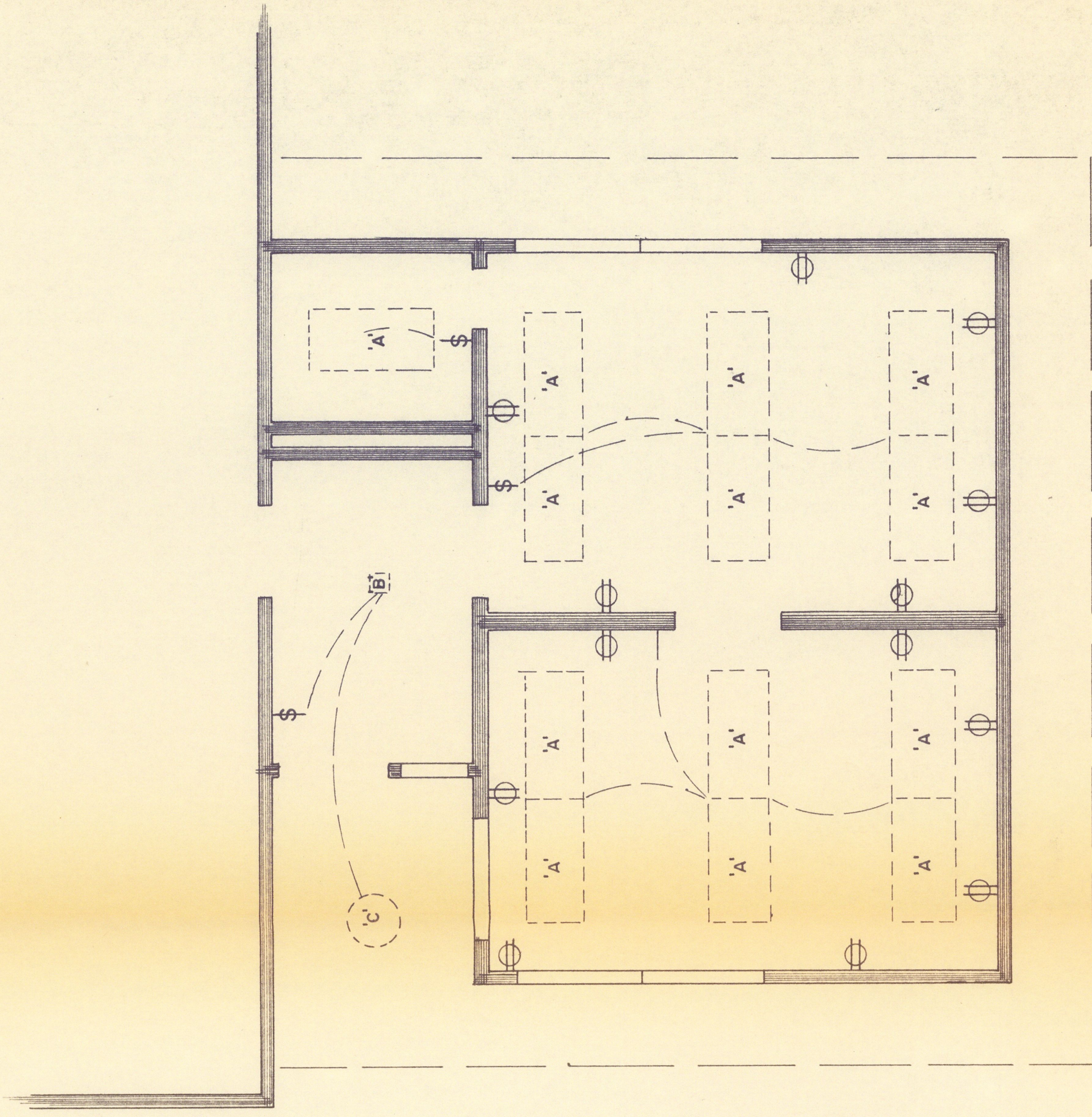
Office Electrical Layout
