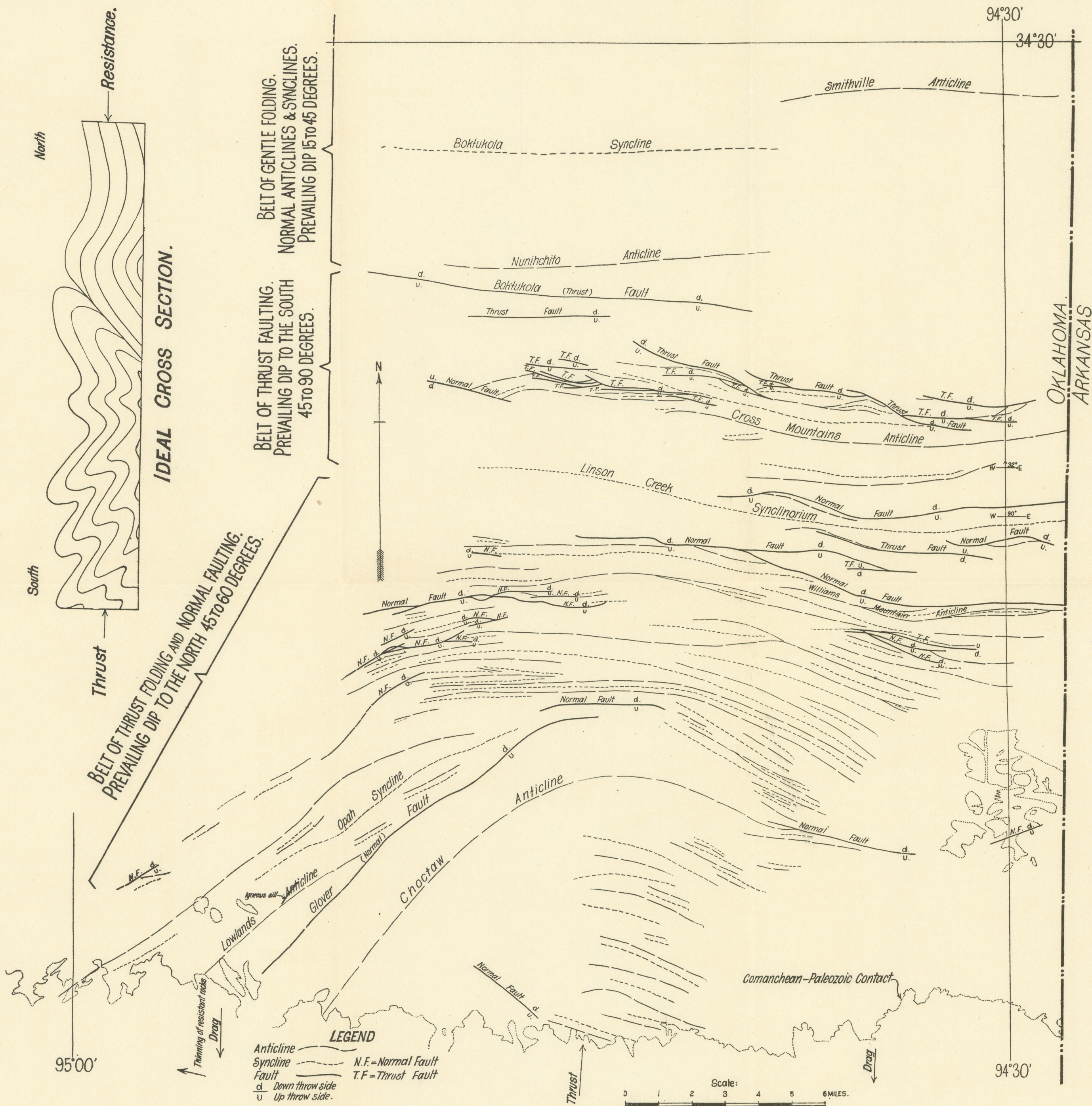
MAP SHOWING ESSENTIAL STRUCTURAL FEATURES AND IDEAL NORTH-SOUTH CROSS-SECTION OF THE AREA
