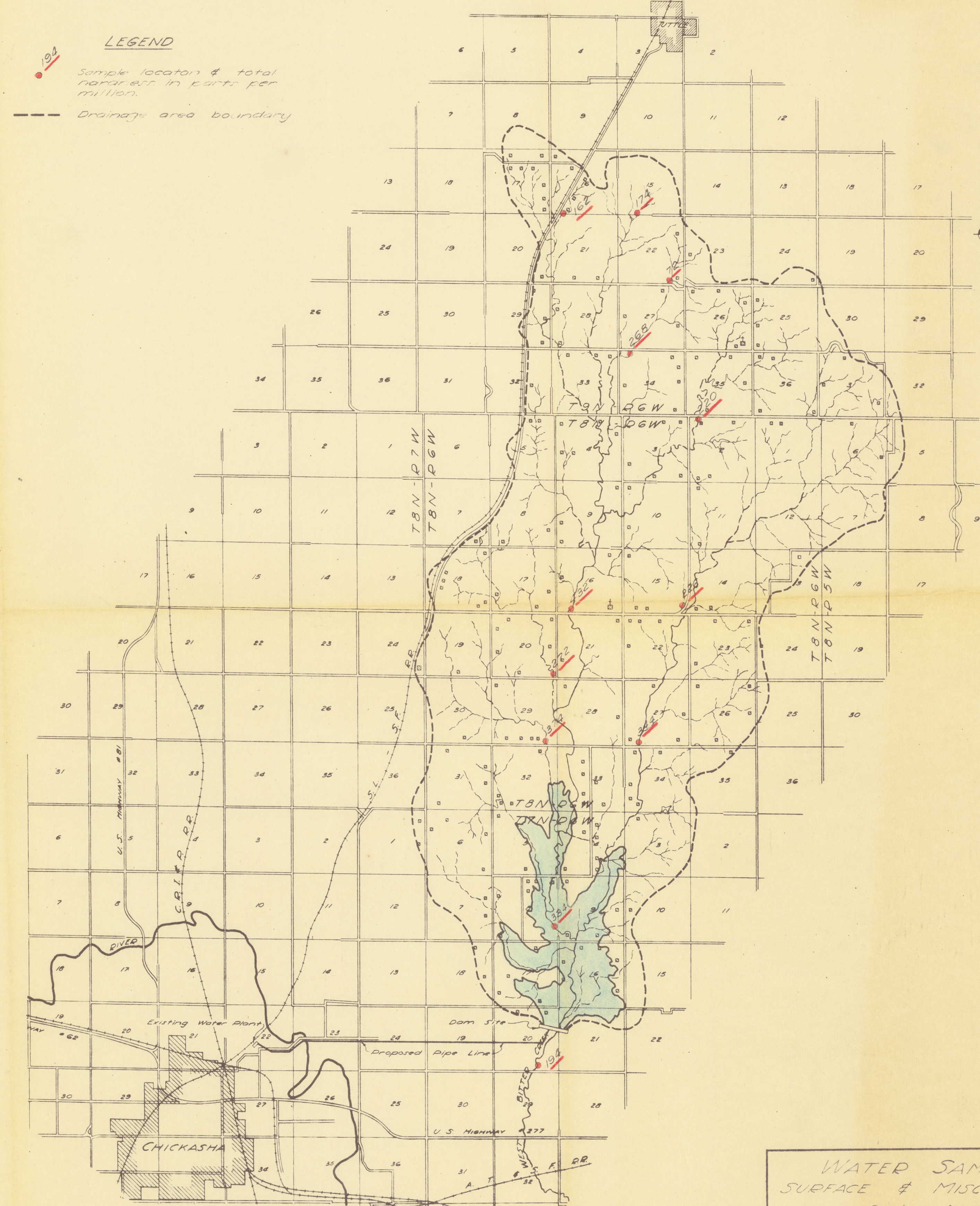
PLAT SHOWING RESERVOIR SITE, DRAINAGE AREA, AND RELATION TO EXISTING WATER FILTRATION PLANT Scale 1" = 1 mile
